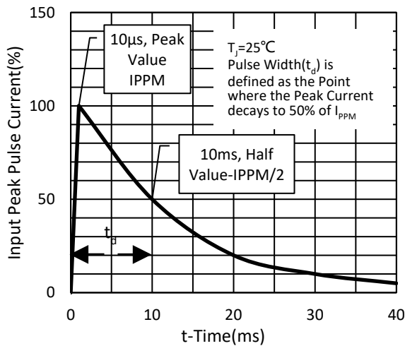
Fig.3 – Pulse Waveform
